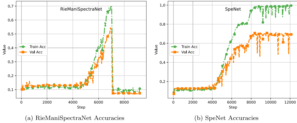
Fig. 9. Plots of the average accuracy profiles during the training process. Both case studies (a) and (b) show the accuracy calculated during training on the training set (Train Acc) and the validation set (Val Acc). It can be seen, as in Fig. 8, that the performance of RieManiSpectraNet collapses quickly after reaching the optimum value, unlike the performance of SpeNet. This is taken as an index of the difficulty of training the proposed RieManiSpectraNet architecture.
